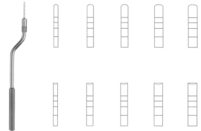
Implants Instruments FI-2292 Fig.1B 165mm
